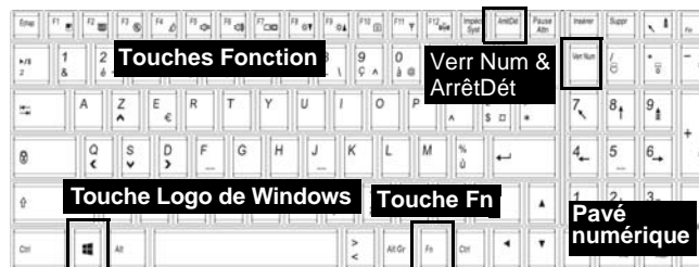
Figure 6 - Clavier
