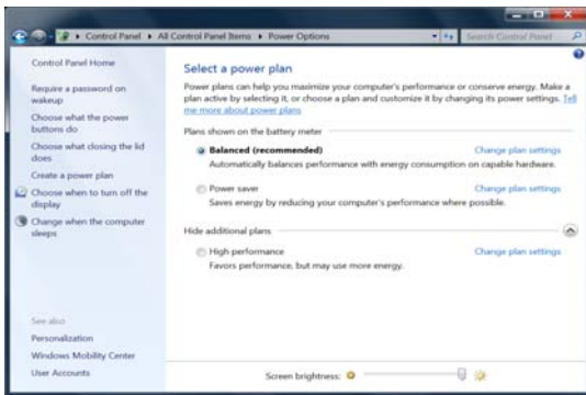
Figure 15 - Power Options
