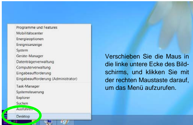
Abb. 11 - Kontextmenü (Windows 8)
