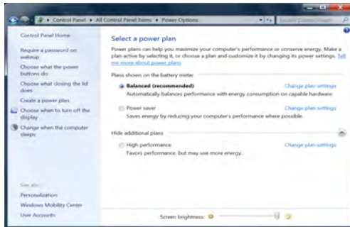
Figure 15 - Power Options
