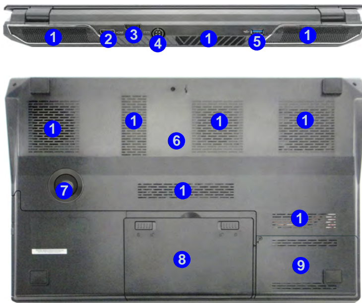
Figure 10 - Rear & Bottom Views
